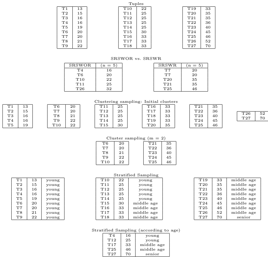
Figure 2.7: Examples of sampling: SRSWOR, SRSWR, cluster sampling, stratified sampling.
