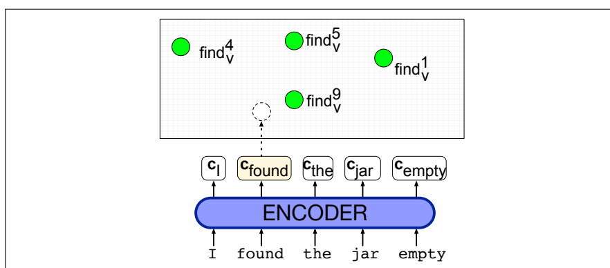
Figure 23.9 The nearest-neighbor algorithm for WSD. In green are the contextual embeddings precomputed for each sense of each word; here we just show a few of the senses for find . A contextual embedding is computed for the target word found , and then the nearest neighbor sense (in this case \text{find}_v^9 ) is chosen. Figure inspired by Loureiro and Jorge (2019).
