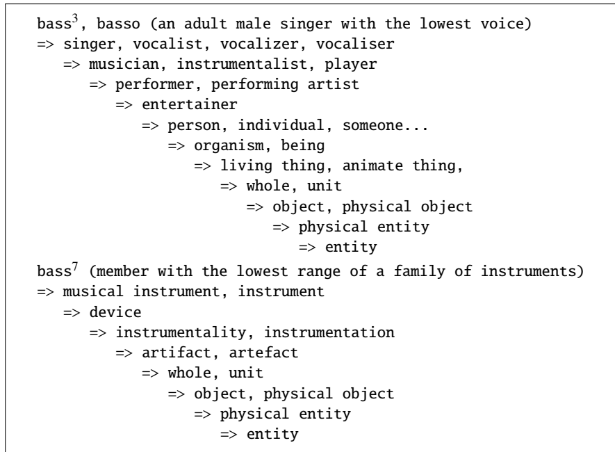
Figure 23.5 Hyponymy chains for two separate senses of the lemma bass . Note that the chains are completely distinct, only converging at the very abstract level whole, unit .
